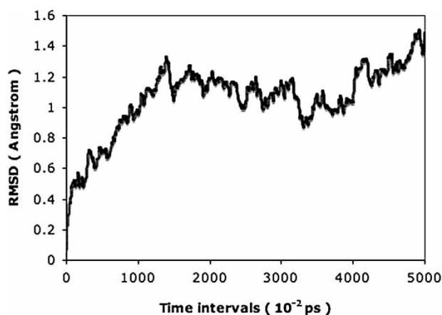
Figure 3. RMSD of ssDNA backbone in NVT ensemble.
