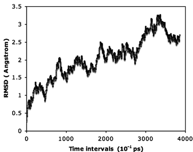
Figure 4. RMSD of ssDNA backbone in NPT ensemble.
