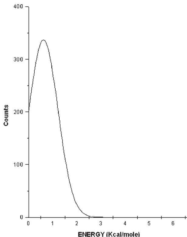
Figure 2. The distribution of kinetic energy of ssDNA system in NVT ensemble.
