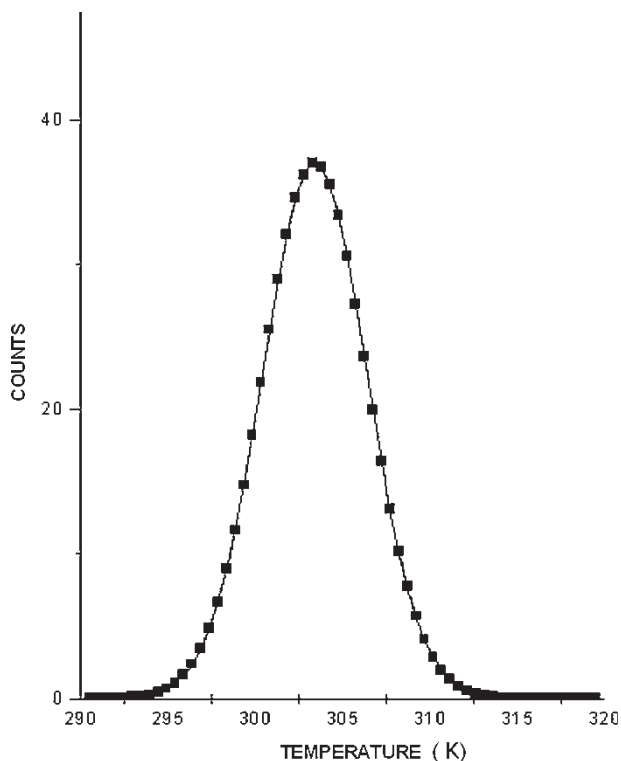
Figure 1. Temperature fluctuation observed in NVE ensemble of ssDNA.
